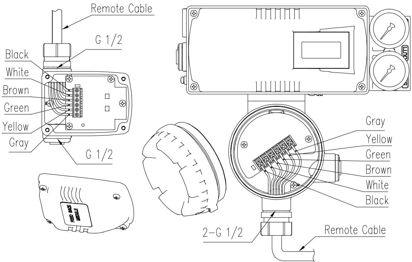
图5-3: YT-3702遥感器及接线盒概览端子概览
